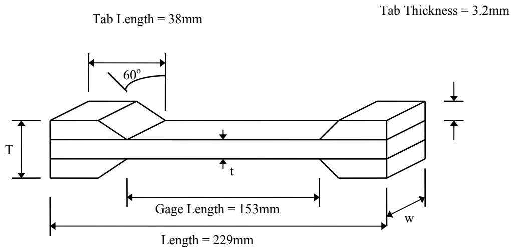
Figure 1 Schematic of Test Specimen used to find the Young's modulus of a composite.
