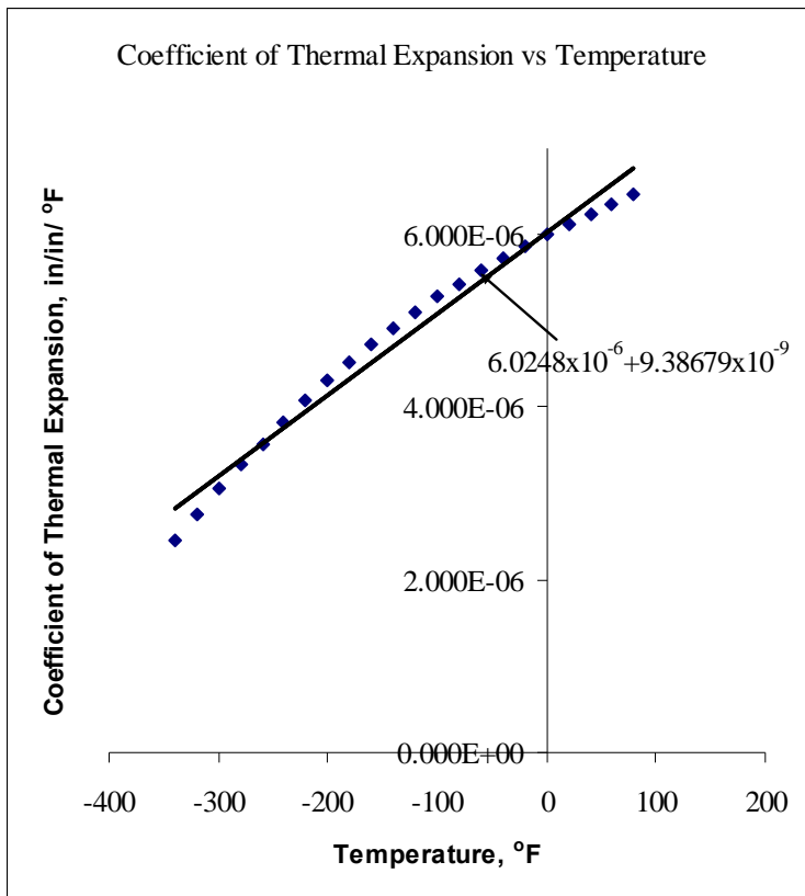
Figure. Linear regression of Coefficient of Thermal expansion vs. Temperature data
