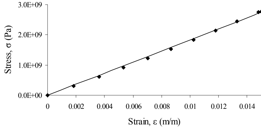
Figure 5 Linear regression model of stress vs. strain for a composite material.
