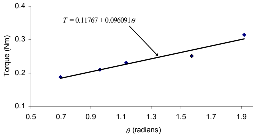
Figure 4 Linear regression of torque vs. angle data
