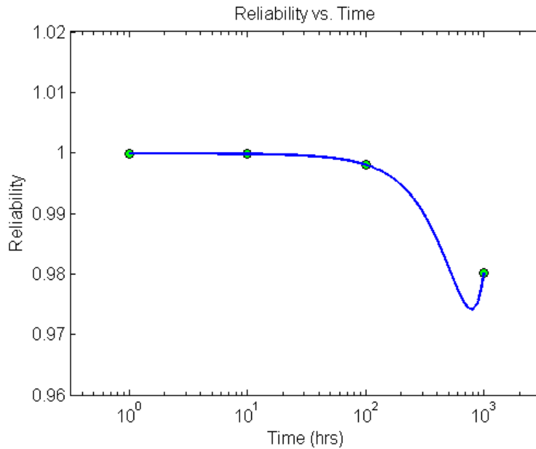
Figure 2 Graph of reliability as a function of time.
