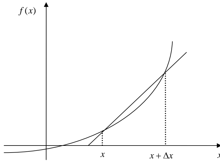
Figure 1 Graphical representation of forward difference approximation of first derivative.
